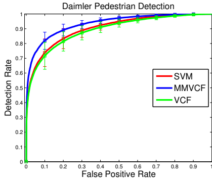
Figure 2. ROC curve of detection rate vs false positive rate comparing MMVCF, SVM and VCF for pedestrian detection
