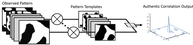
Figure 1. The outputs of each feature channel are aggregated to compute the final correlation output which is desired to have a sharp peak at the object location for the correct object class.
