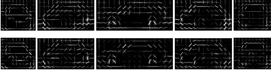
Figure 6. Visualization of the learned root filters for five car poses. Top Row: HOG SVM. Bottom Row: HOG MMVCF.
