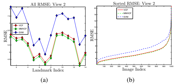
Figure 3. a) RMSE of 14 landmarks averaged over all images. b) Comparison of sorted RMSE for different landmark detectors.
